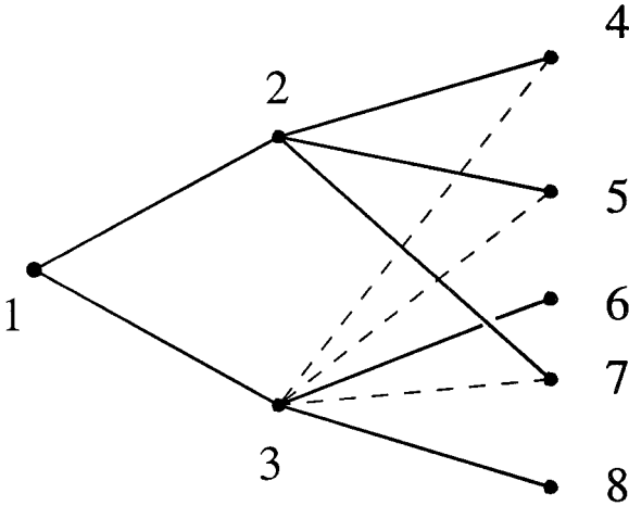
Fig. 1. A tree T on \mathbb{N}_8 (solid lines). The dashed lines are those lines of H^*(T) that connect V_1 = \{2, 3\} to V_2 = \{4, 5, 6, 7, 8\} .
